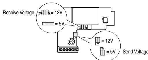
Figure 1.13 Jumper Settings
