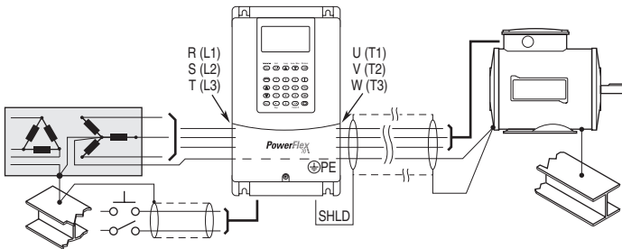
Figure 1.1 Typical Grounding
